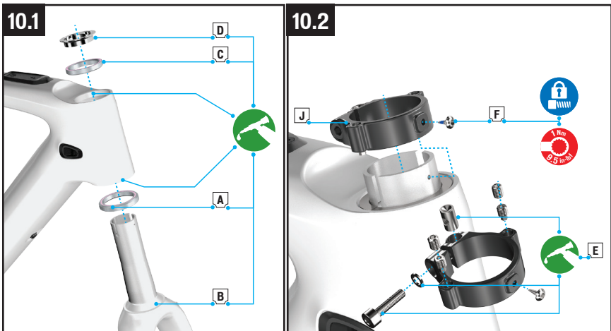
Fig.10.1: Grease, then install the lower bearing (A) on the fork (B). Insert the fork into the head tube, then grease and install the upper bearing (C) and compression ring (D) on the steerer tube.
